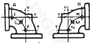
90° ELBOW REDUCING SIZE
