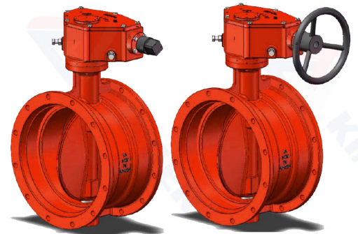
With Wrench Nut With Hand Wheel 10"-24"
